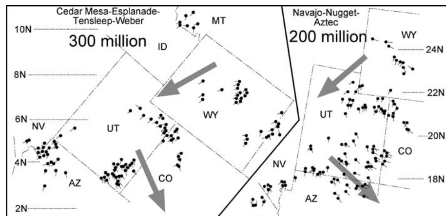
Fig. 2. Dip directions of cross-strata of Late Paleozoic (left) and Early Jurassic (right) eolian sandstones. Tails of “tadpoles” point downwind; each represents scores of measurements. Large gray arrows show the flow of trade winds (top arrows) and tropical westerlies (bottom arrows). Paleomagnetic data indicate that, during the Permian, Utah was near the equator but that, by the Jurassic, it had drifted to 20°N. [Modified from Peterson (7)]
