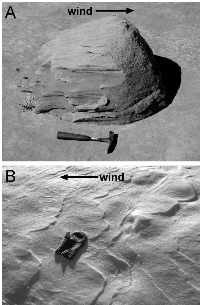
Figure 6. A , Ventifact developed on bedrock knob that is 10 m above and 100 m south (upwind) of the Wave (see fig. 1 B for location). Sand-bearing southwesterly winds blow left to right. B , Wind-eroded forms cut into snow are similar in form and scale to the treads and risers developed on Navajo Sandstone outcrops at the Wave. Note, however, that each riser is developed on a distinct depositional lamina; depositional laminae do not control the position of the sandstone risers (cf. fig. 2 B ). Mitten is 25 cm long.
