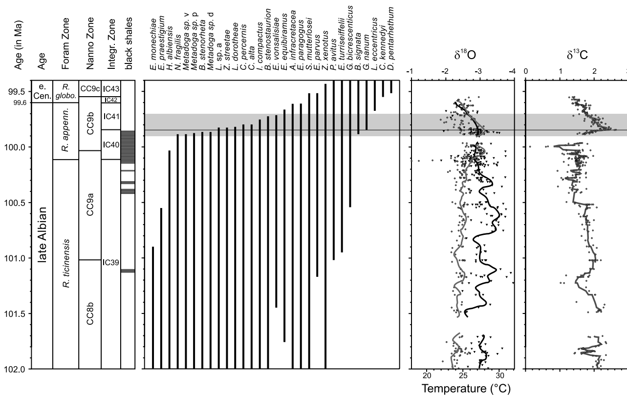
Figure 2. Biostratigraphy of selected taxa from ODP Leg 171B. Age assignments are based on Wilson and Norris [2001] recalibrated by setting the Albian/Cenomanian boundary at 99.6 Ma. Foraminiferal biostratigraphy is from Bellier et al. [2001]. The distribution of laminated black shale facies, based on data from Norris et al. [1998], is illustrated by horizontal shading. Nannofossil species are plotted as range-through distributions. Oxygen and carbon isotope data are from Wilson and Norris [2001]. Black lines indicate the five-member moving average of isotopic values from thermocline-dwelling species, while the shaded line indicates the moving average of surface-dwelling planktonic foraminifers. The interval of increased extinction (from 99.7 to 99.9 Ma) is indicated by a shaded horizontal band. The level of the maximum positive carbon values in the positive excursion is indicated by a horizontal black line.
