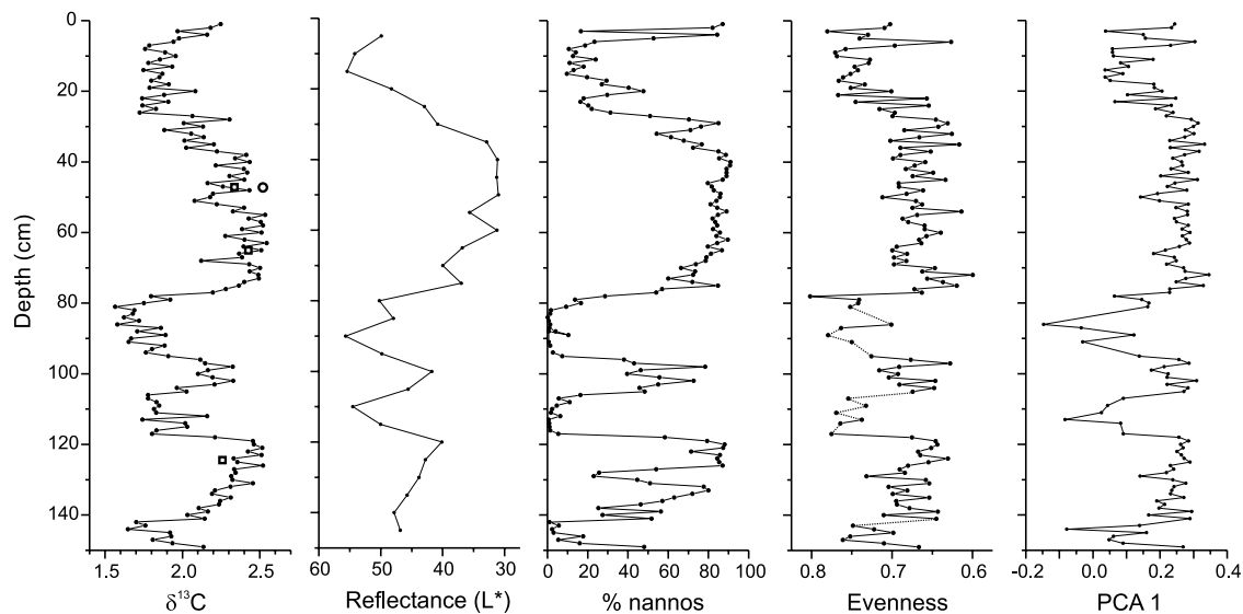
Figure 5. Distribution of carbon isotope values, reflectance, and nannofossil indices in ODP Section 1052E-39R-5. Note that values on the y axis for reflectance and nannofossil evenness have been reversed to allow direct comparison with other distributions. Carbon isotope values, plotted as small solid circles connected by line segments, are measured on bulk carbonate. Four \delta^{13}\text{C} values measured from discrete, “glassy” well-preserved planktonic foraminiferal calcite in the clay stones [Wilson and Norris, 2001] are included for comparison. Three of these discrete values (indicated by squares) are from thermocline-dwelling species, whereas the fourth value (indicated by large open circle) is from a surface-dwelling taxon.
