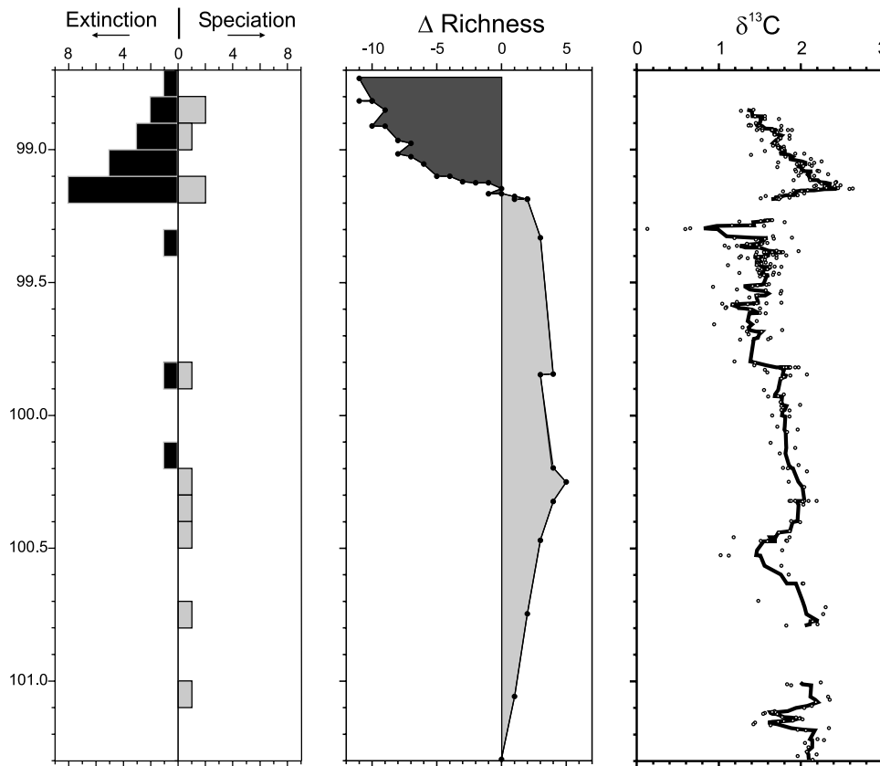
Figure 3. Evolutionary changes in species richness. Distribution of speciation and extinction events is based on stratigraphic ranges compiled in Figure 2. Cumulative changes in species richness ( \Delta Richness) indicate significant interval of extinction is coincident with a large positive carbon isotopic excursion.
