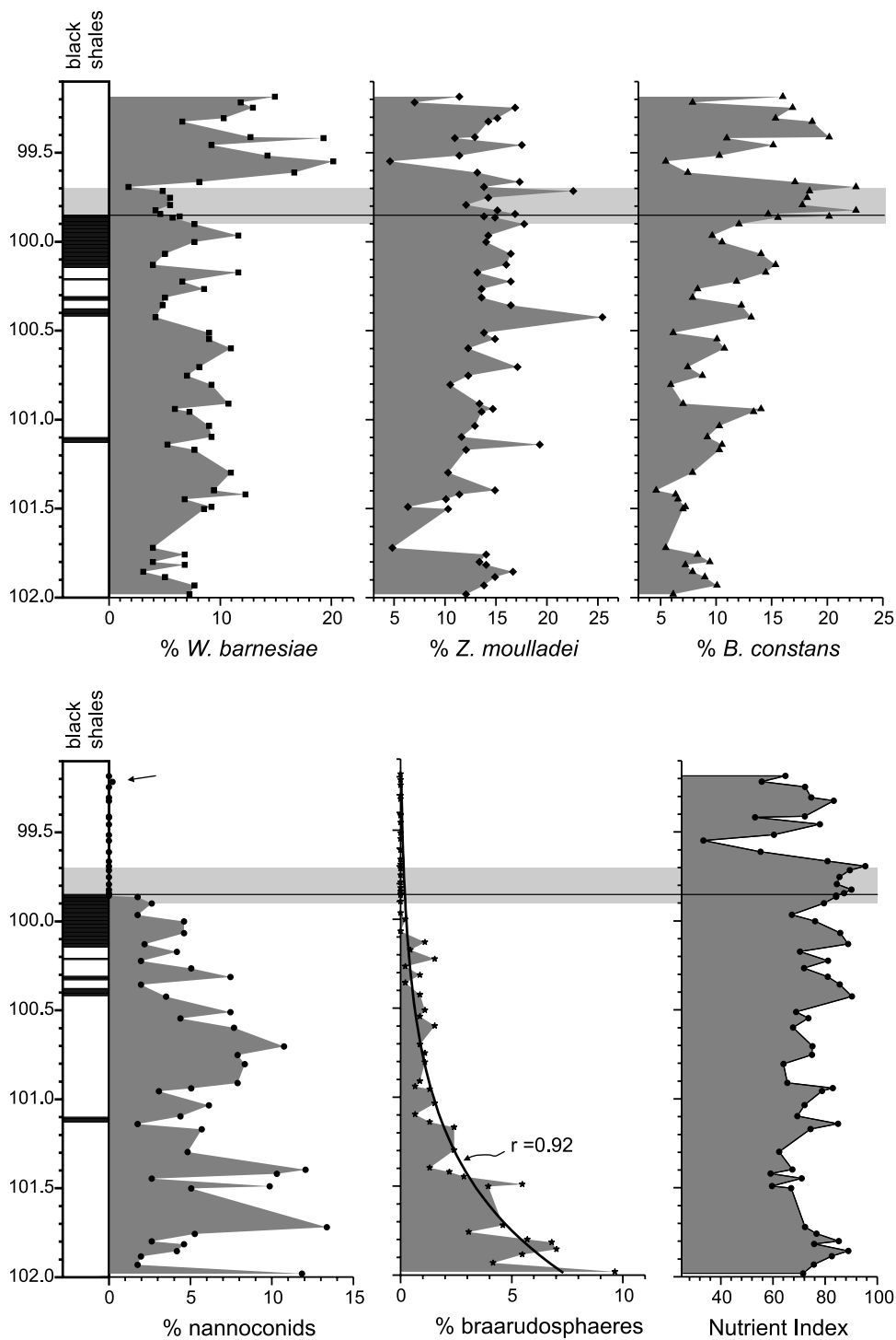
Figure 4. Abundances of major taxa and the nutrient index from the Blake Nose. Disjunct occurrence of nannoconids is indicated by arrow. The distribution of laminated black shale facies, based on data from Norris et al. [1998], is illustrated by horizontal shading. The interval of increased extinction (from 99.7 to 99.9 Ma) is indicated by a lighter shaded horizontal band. The level of the maximum positive carbon values in the positive excursion is indicated by a horizontal black line.
