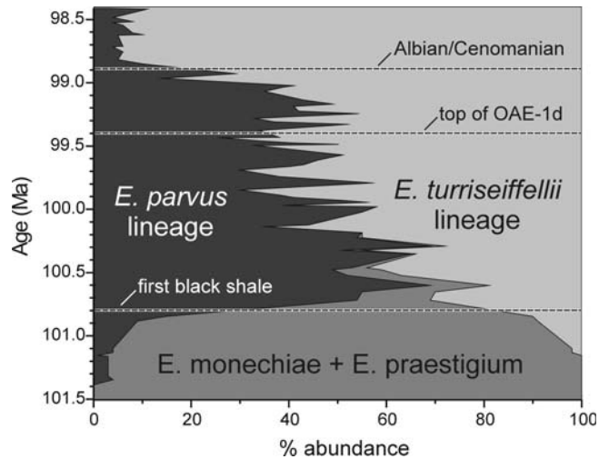
TEXT-FIGURE 9 Distribution of the three major groups of upper Albian eiffellithids and their relationship to the onset of black shale deposition and the Albian/Cenomanian boundary.
