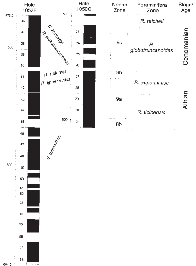
TEXT-FIGURE 2 Biostratigraphy of the study interval from ODP Holes 1050C and 1052E. For each hole, from left to right, are the depth in meters below sea floor, core number, and core recovery (with black indicating recovered core and white indicating empty core barrel). The nanofossil zonation is based on unpublished data of Watkins and is correlated to the zones of Perch-Nielsen (1985). The foraminiferal zonation is from Bellier et al (2001).
