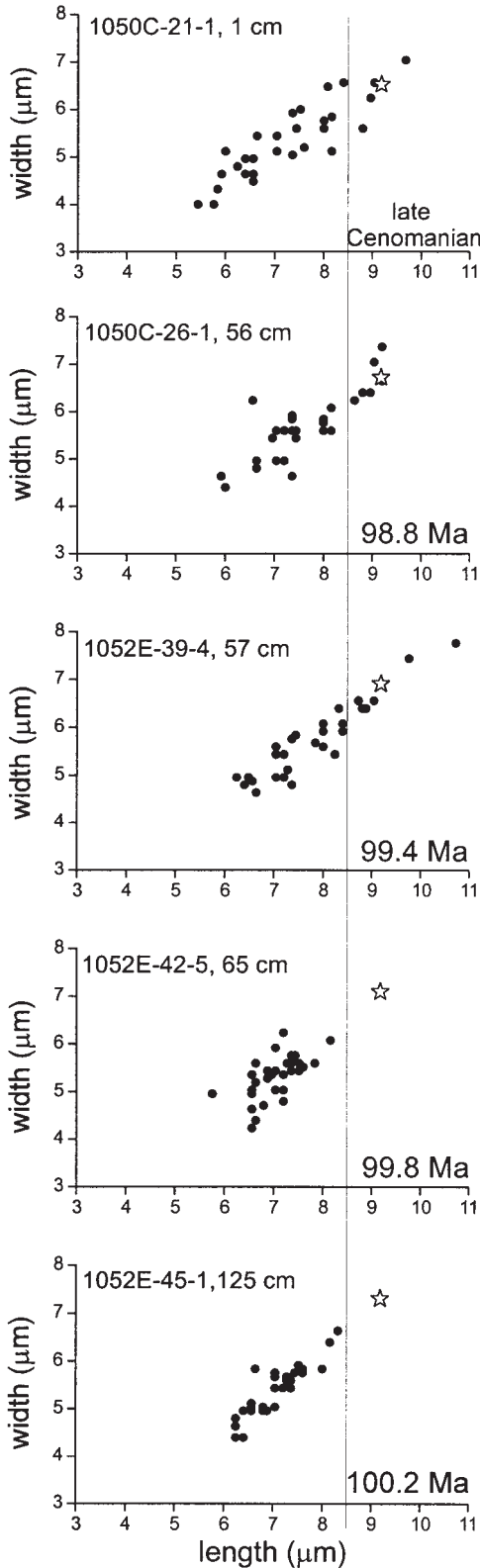
TEXT-FIGURE 5 Length vs. width relationship for five samples of E. turriseiffelii . Note that the samples from older populations (100.2 and 99.8 Ma) contain only forms smaller than 8.5µm in length, while later ones contain the larger morphotypes. The star in each graph indicates the size of the holotype for E. turriseiffelii .
