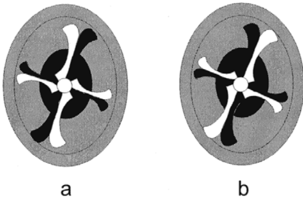
TEXT-FIGURE 10 Schematic diagram illustrating the shift of birefringence that results in the “trick” in the cross polarized images of E. praestigium .
