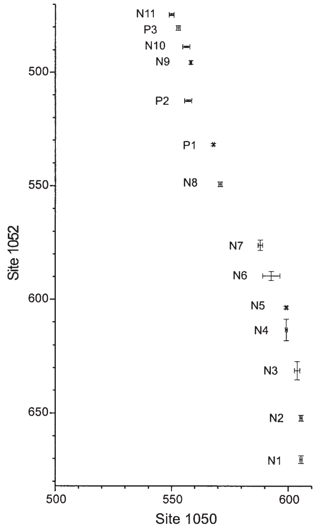
TEXT-FIGURE 6 Graphic correlation of Sites 1050 and 1052, based on the biostratigraphic distribution of the eiffellithids and planktonic foraminifers. Data for this graph are compiled in Table 3.
