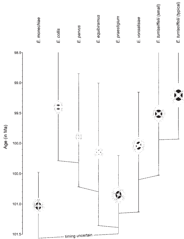
TEXT-FIGURE 3 Proposed calibrated range chart.
