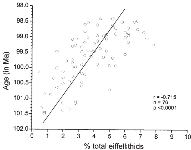
TEXT-FIGURE 8 Eiffellithid abundance through time. This illustrates the clear trend towards increasing importance of the genus during the late Albian and early Cenomanian. Once attained, the high relative abundance of eiffellithids is generally maintained throughout the rest of the Cretaceous.
